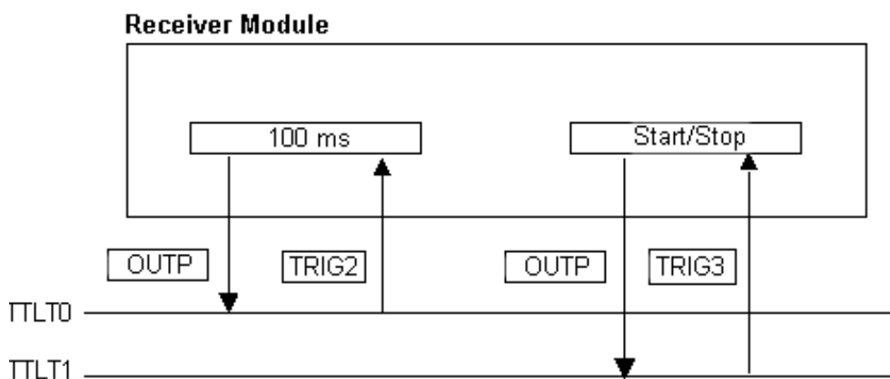
Figure 7-1. Trigger System
